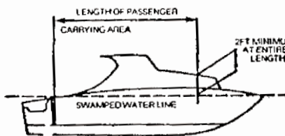
FIGURE 6. BOAT WITH CABIN
