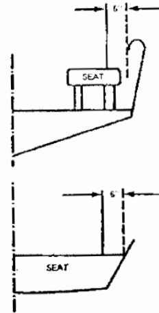
FIGURE 13. LOCATION OF CENTER OF GRAVITY OF WEIGHTS ON SEATS
