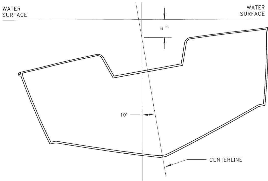
FIGURE 5.8 Flotation Test
